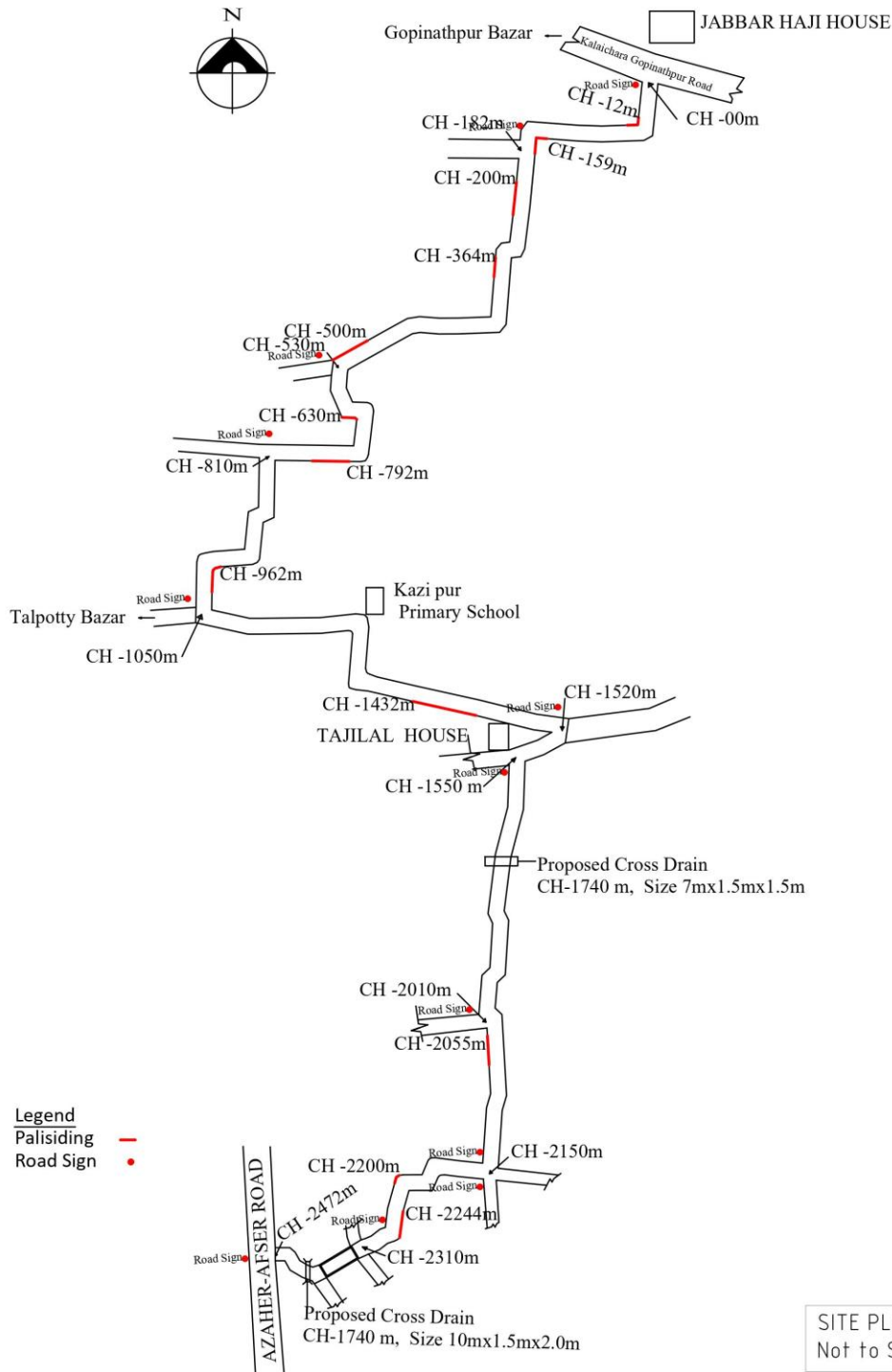
Layout Plan
